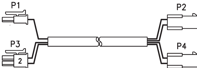
Figure 5 Twin Cable Extension
